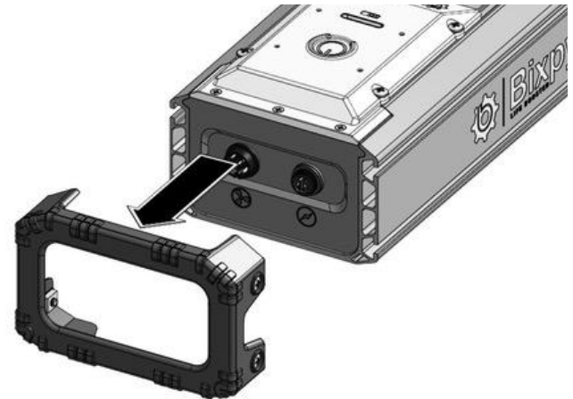
STEP 2: Slide the bumper off the battery shell
