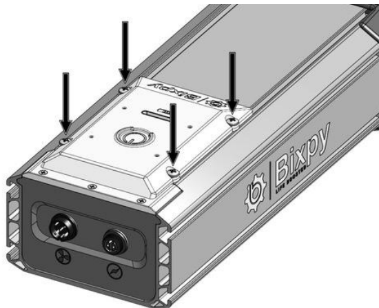
STEP 3: Loosen the Controller Module screws
