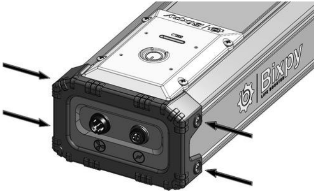
STEP 1: Loosen or remove the bumper screws
